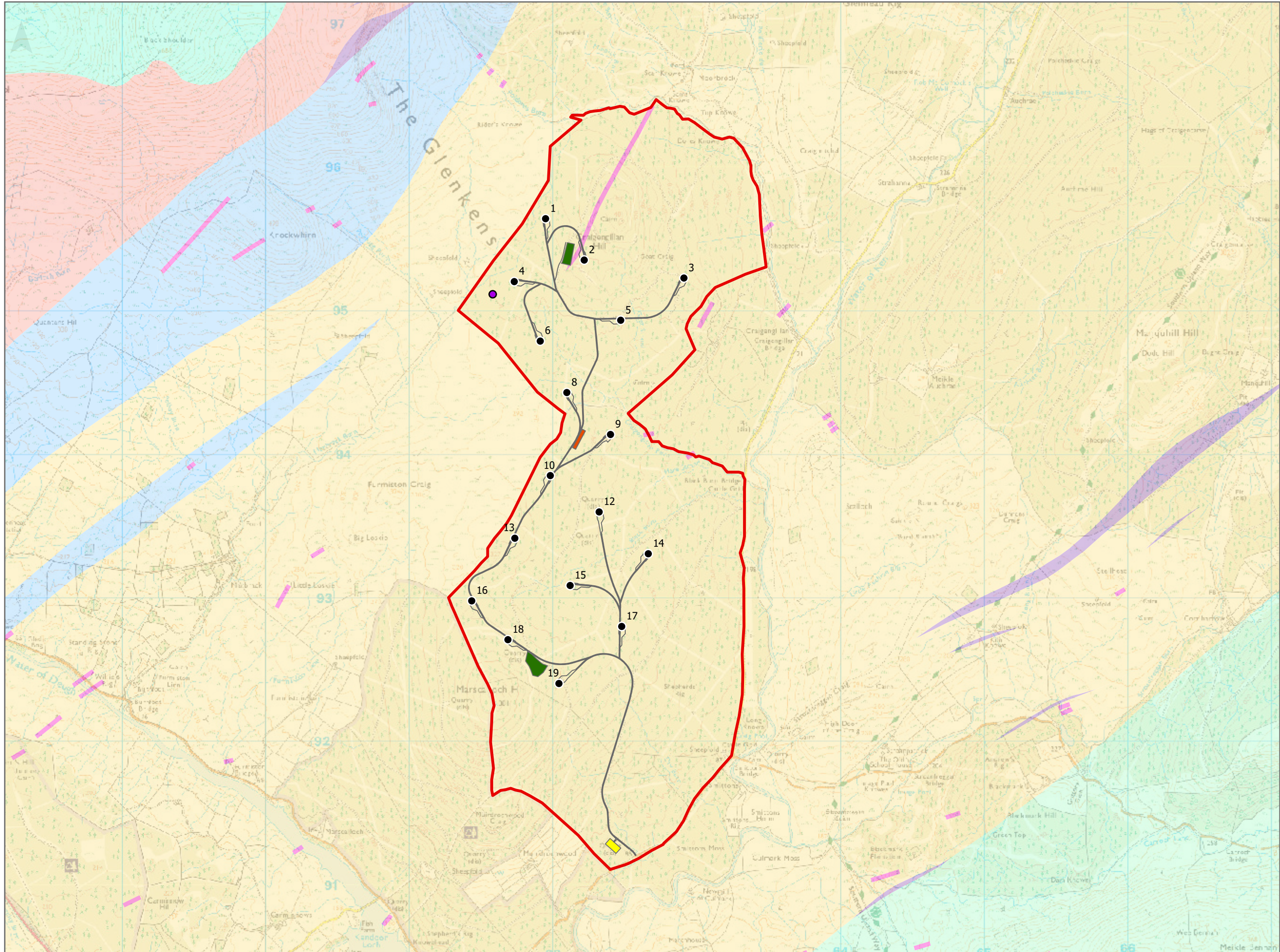
Figure 12.2: Bedrock Geology
